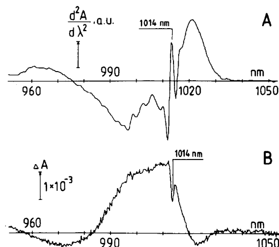
Fig.3. (A) Second derivative of the absorption spectrum of Rps. viridis RCs at 1.7 K after illumination for 1 h in state CytHMPI - Q - (reaction 3) at 1014 nm and 1.7 K. (B) Difference between two absorption spectra of the same RCs measured at 6.5 and 13 K.
