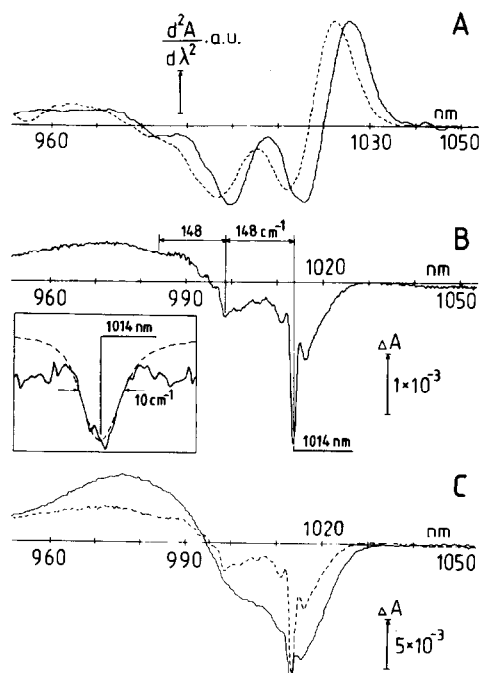
Fig.2. (A) Second derivative of the absorption spectrum of Rps. viridis RCs in the normal (CytPIQ) state (solid) and in state CytPI - Q - (dashed) measured at 1.7 K. (B) Same as A but for reaction 3: CytHMPI - Q - → Cyt + HM - PI - Q - . Illumination time, 15 min. (Inset) Shape of burned hole with greater spectral resolution (solid) and profile of Hg line at 1014 nm measured under the same optical conditions (dashed). (C) Same as B after subsequent illumination with white light (10 mW/cm 2 ) for 10 min at 1.7 K (solid). The bar refers to the solid line. Dashed line shows the spectrum of B, normalized with solid curve at 1014 nm.
